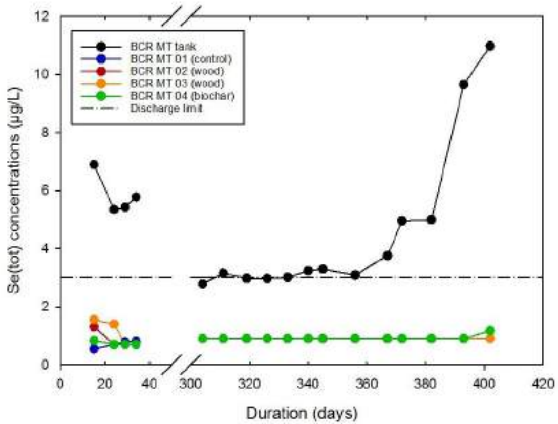
Figure 5. Selenium concentration in influent and effluent of the four bioreactors (BCR-MT-01 to -04) between August 20 th 2014 and September 26 th 2015 (Discharge Limit of 0.003 mg/L).
